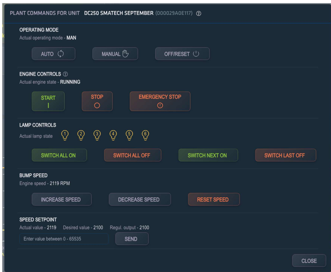
Example of available Plant Commands on DC250 in Ligting Tower Mode
